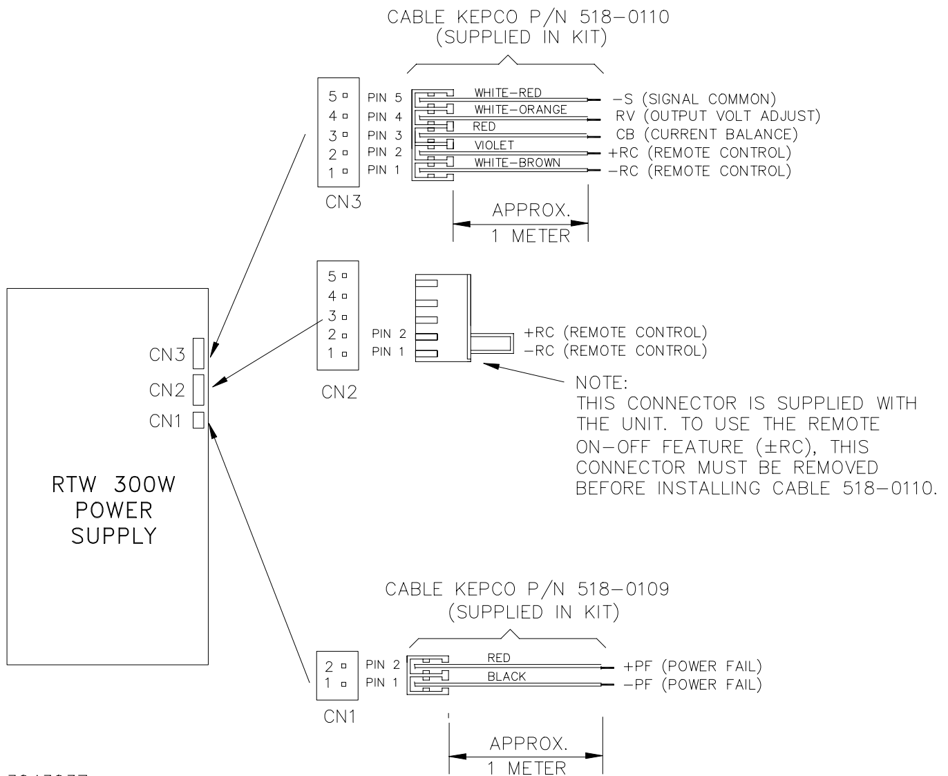
FIGURE 1. CABLE KIT INSTALLATION
